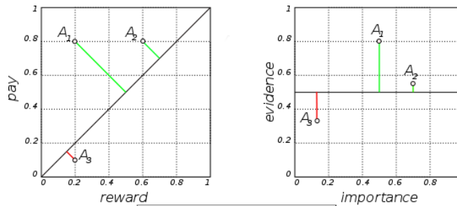
Figure 2: Belief values can be expressed either as an evidence-imp pair or as a pay-reward pair. The diagonal (left) represents evidence = 0.5, meaning doubt. The area left-above the diagonal represents positive beliefs with evidence > 0.5; the area right-under the diagonal represents negative beliefs (evidence < 0.5). See Example 1 for more details about the beliefs of agents A 1 , A 2 and A 3 .
